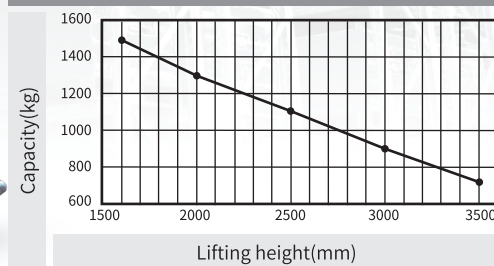
CAPACITY CHART
